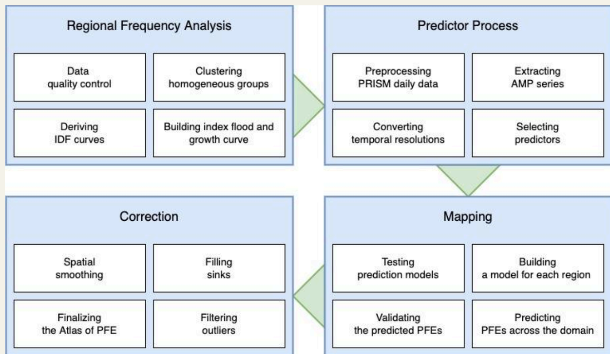
Figure 3.1. A framework to develop a precipitation frequency estimate map
