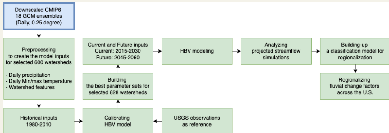
Figure 4.2. A workflow of creating fluvial change factors
