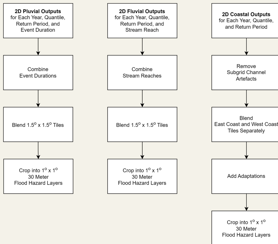
Figure 2.10. A workflow of the inland and coastal post-processes
