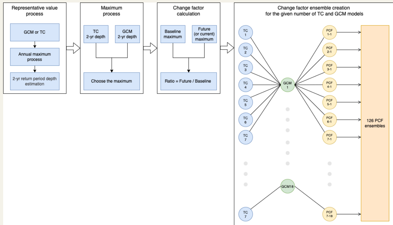
Figure 3.4. A workflow of the PCF ensembles creation
