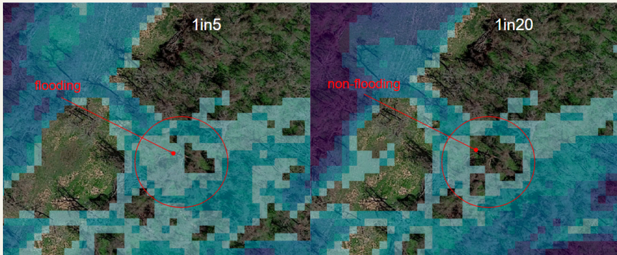
Figure 2.12. Before monotonicity: flooding appears in a 5-year return period but not a 20-year
