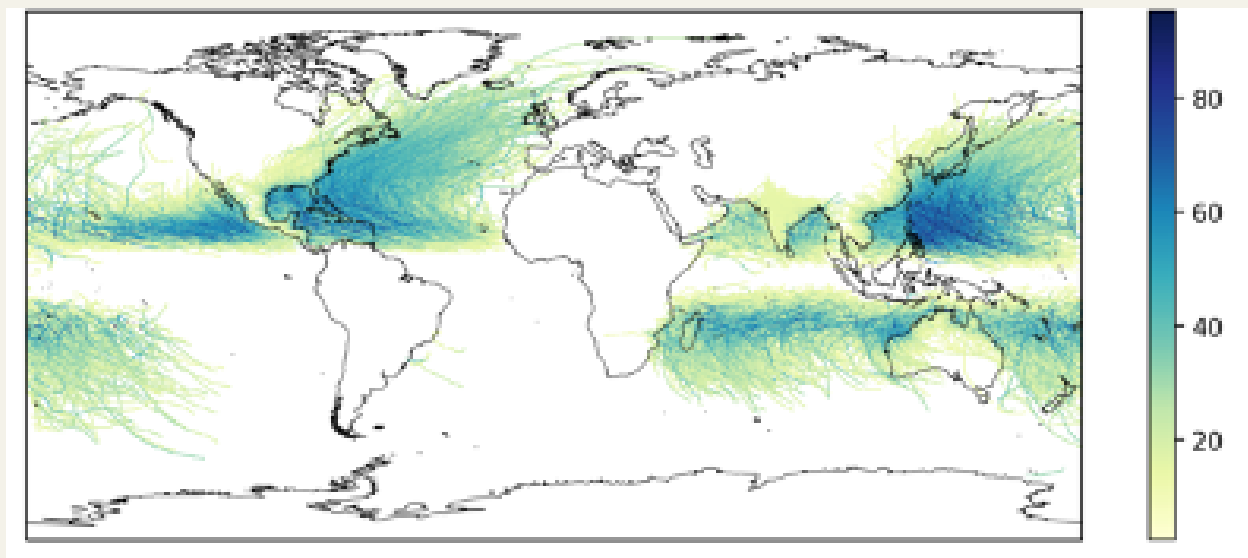
Figure 2.2. Maximum 1-minute sustained wind speeds (Meters per second) for historical global tropical cyclone tracks
