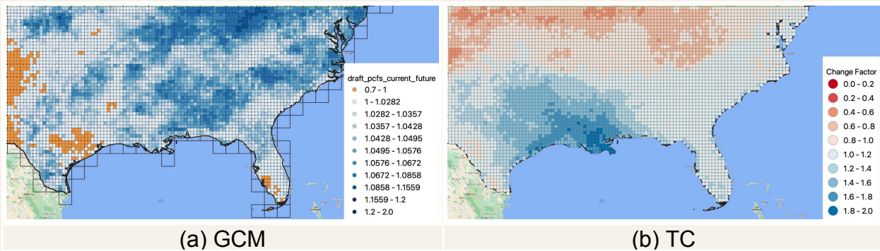
Figure 3.5. Comparison of the GCM-driven and TC-driven PCF distributions in the TC region: An example of specific GCM and TC models
