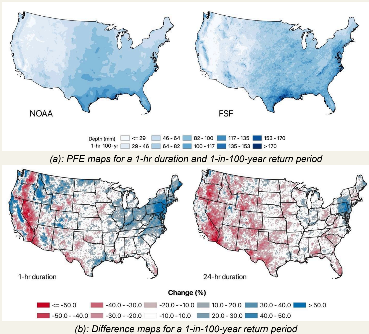
Figure 3.2. Comparison of maps of PFEs from the NOAA Atlas and FS-PM. (a) is a comparison of two atlases for a 1-in-100-year return period and 1-hr duration. (b) shows the percent change in the FS-PM compared to the NOAA Atlas 14 for the same return period and 1- and 24-hr durations. The percent change is calculated from a simple equation: (FS-NOAA)/NOAA \times 100 (\%) .
