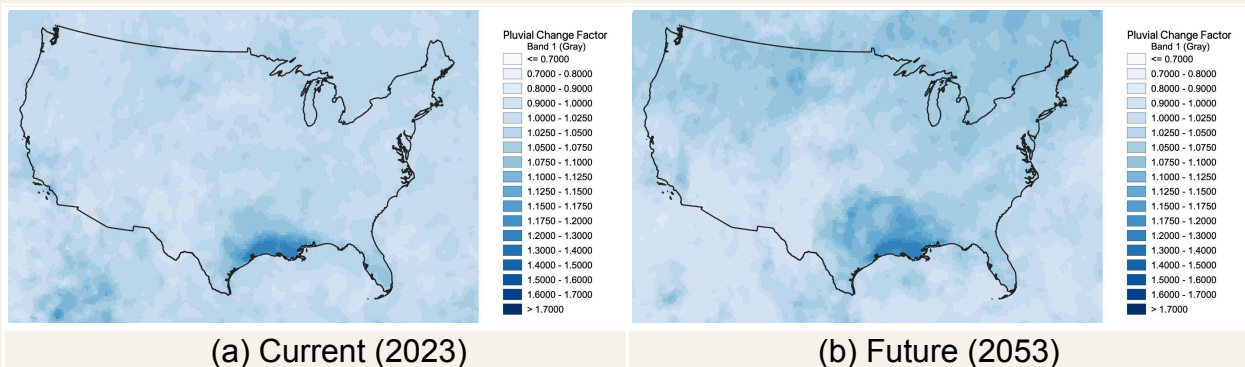
Figure 3.6. Final PCF distributions for the current and future years
