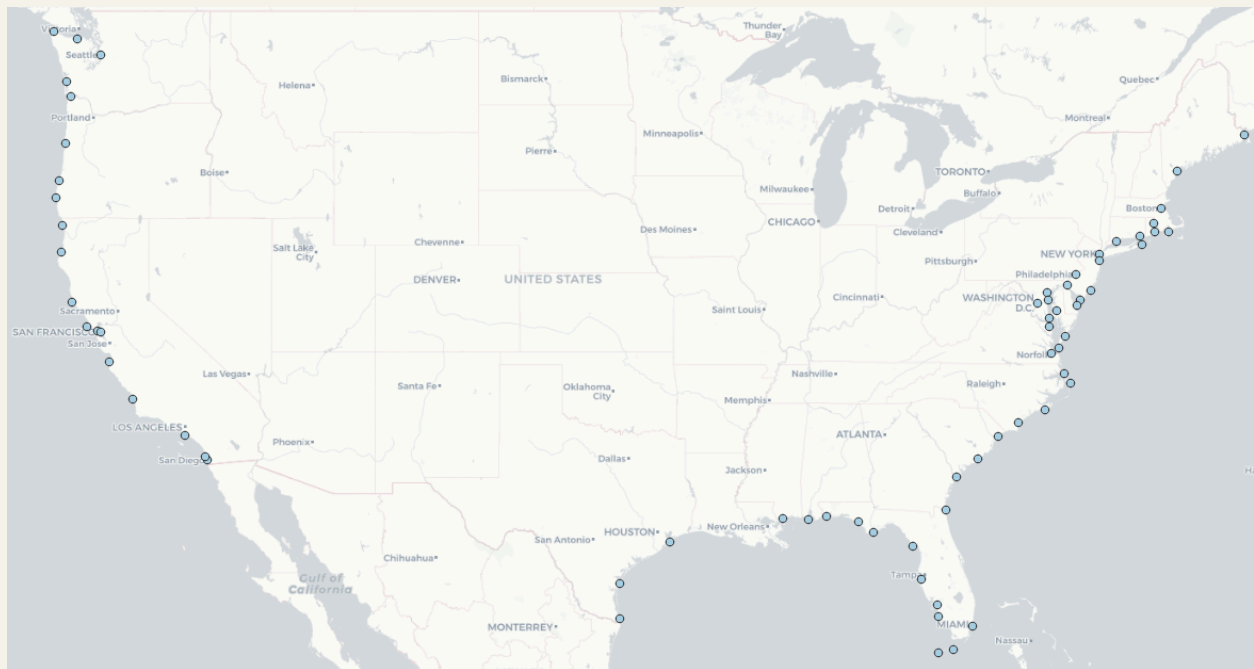
Figure 5.2. A map of the NOAA gauge network
