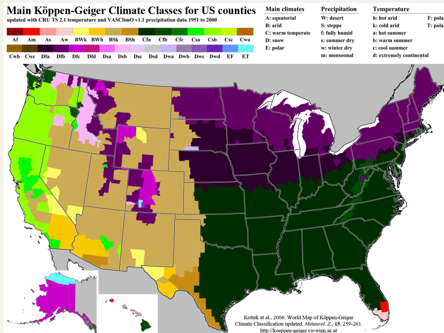
Figure 4.1. Köppen-Geiger climate zones across the Contiguous U.S. (Source: http://koeppen-geiger.vu-wien.ac.at/usa.htm ).
