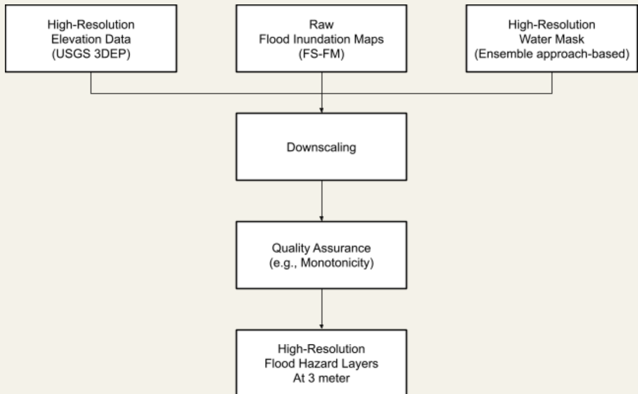
Figure 2.11. A workflow of the downscaling and monotonicity processes
