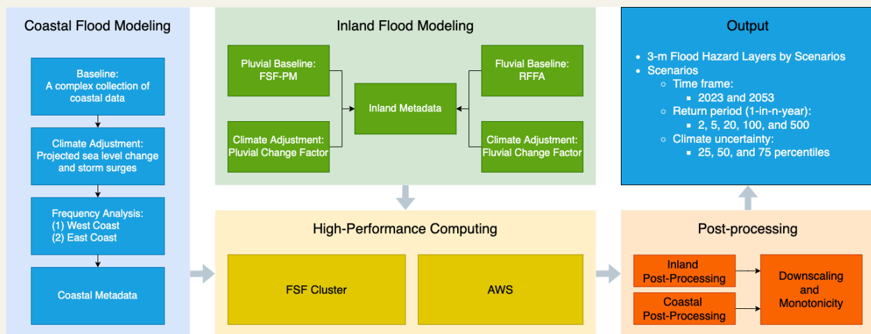
Figure 2.1. A workflow chart of the FS-FM flood model development
